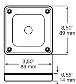
Surface Mount 5600, 5602, 5603
