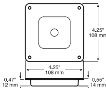
Recessed Mount 5600-1, 5601
