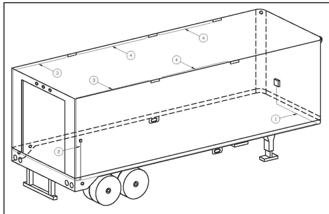
For illustration purposes: 53' trailer kit with rear-mounted timer switch. Includes 5 lights, 8 harnesses and 1 timer switch.
