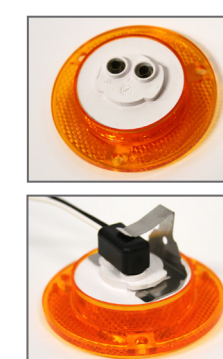
B142-49 PL10 Plug & B162-093 Clip
